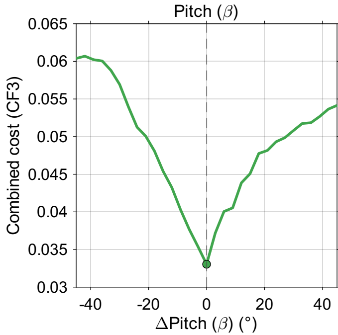
UAV: Angle sensitivity of camera 1 (CA-best, Uniform, sp=1.00 m, 7 cams)
